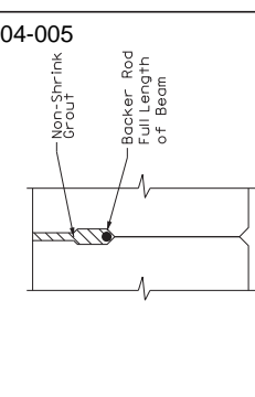
SHEAR KEY DETAIL
