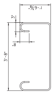
#4S1(E) BAR
